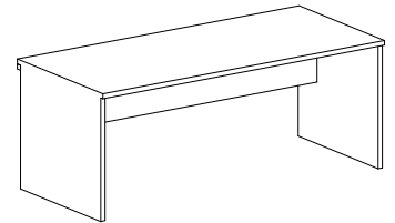
ART.40.04 180x80x75
